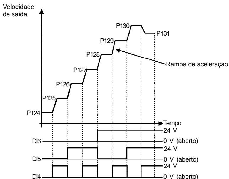
Figura 6.2 - Multispeed
